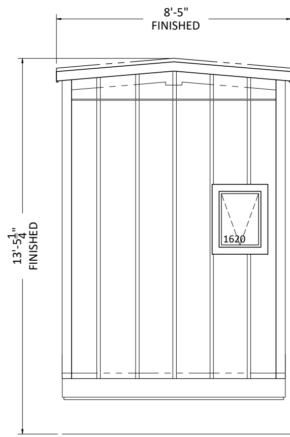
VIEW - AA
