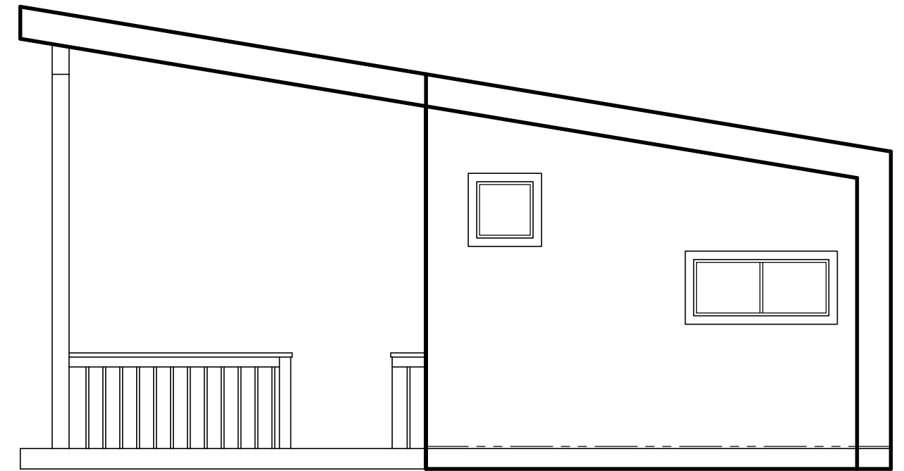
ELEVATION - SIDE GEAR ROOM SHOWN WITH DECK AND ROOF EXTENSION
