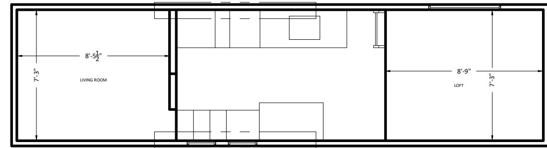
FLOOR PLAN - UPPER
