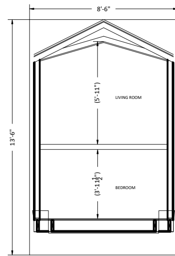
SECTION - REAR
