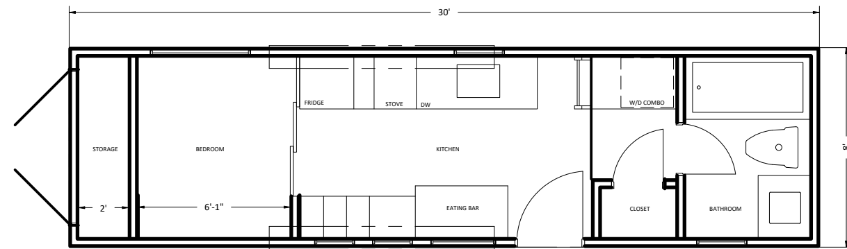
FLOOR PLAN - MAIN
