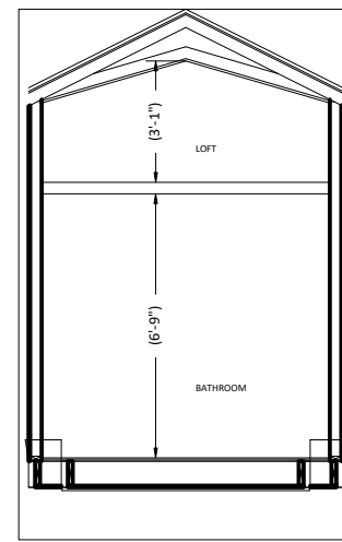
SECTION - FRONT
