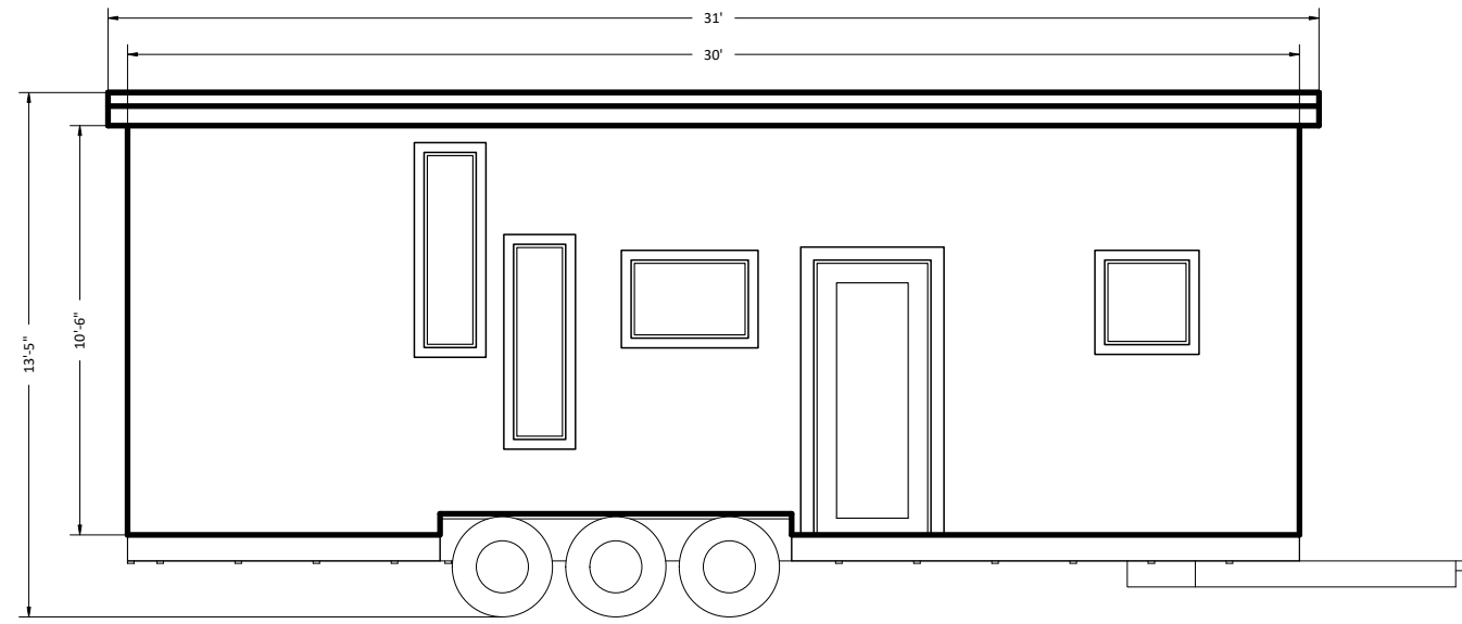
ELEVATION - SIDE
