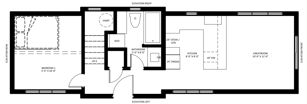
PLAN - MAIN FLOOR
