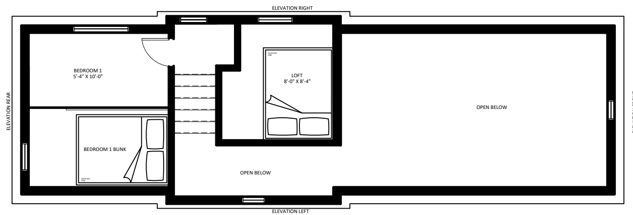
PLAN - TOP FLOOR
