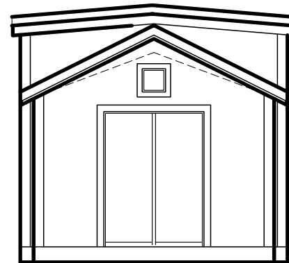
ELEVATION - FRONT
